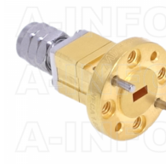
15WECA1.85M_Cu Endlaunch Rectangular Waveguide to Coaxial Adapter 50-65GHz WR15 to 1.85mm Male
