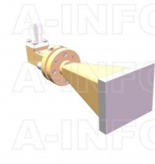
LB-15-20-C-1.85FSPO Standard Gain Horn Antenna 50-65GHz 20dB Gain 1.85mm Female
